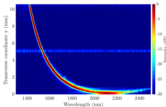
Fig. 2. OPG and OPA wavelength tuning range
