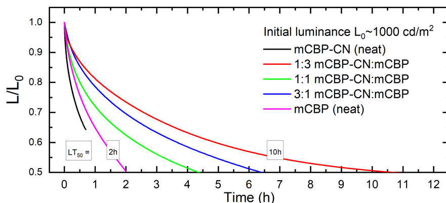
Fig. 1. DMeCzIPN emitter-based OLED luminance vs. time at L 0 ~1000 cd/m 2 initial luminance.
